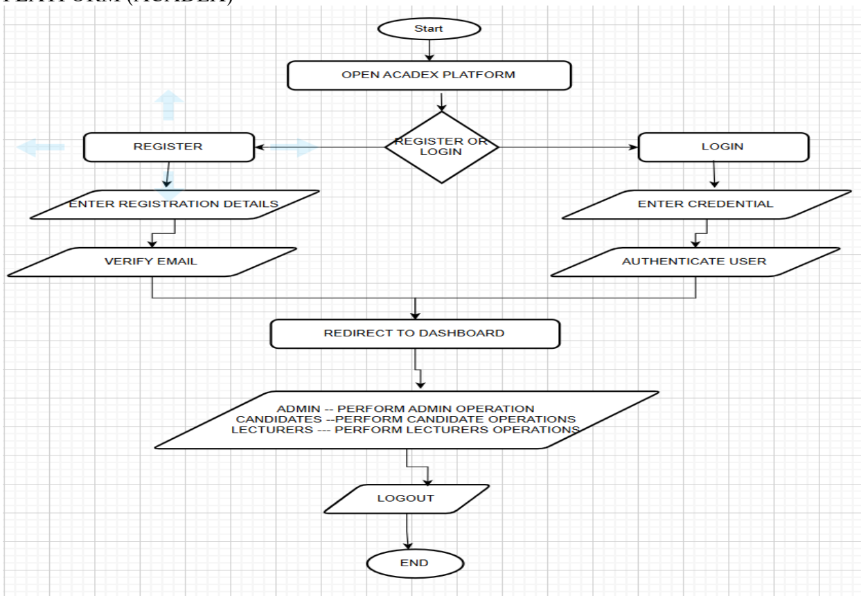
Figure 3 Flowchat Diagram
